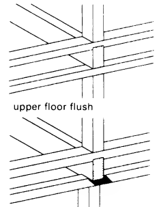
10 Projecting upper floors
